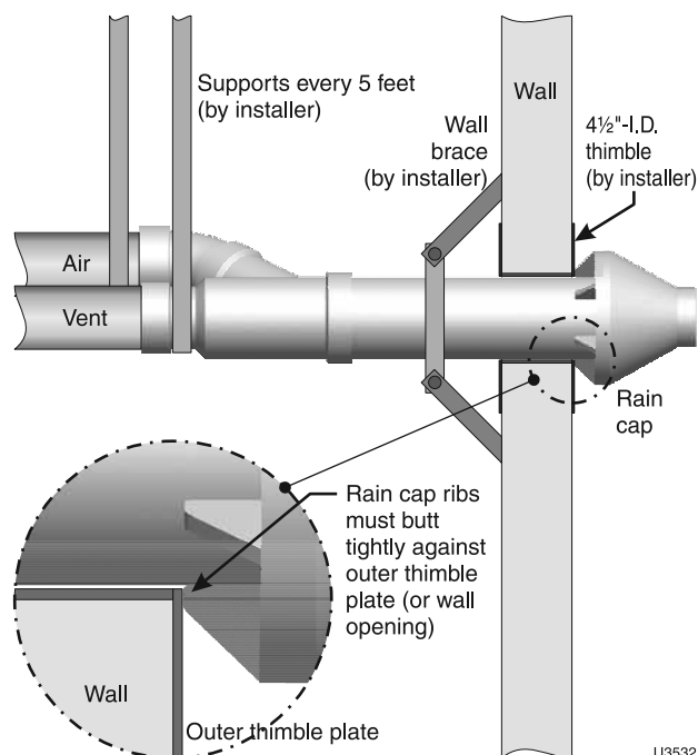
Figure 10 Installing and supporting the concentric sidewall vent assembly
