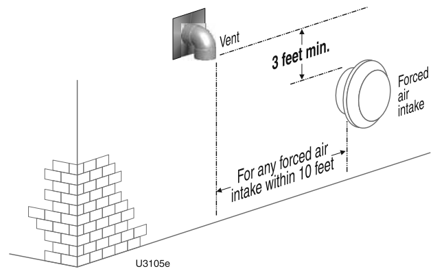
Figure 28 DIRECT EXHAUST — Sidewall — clearances from vent exit to forced air intake
